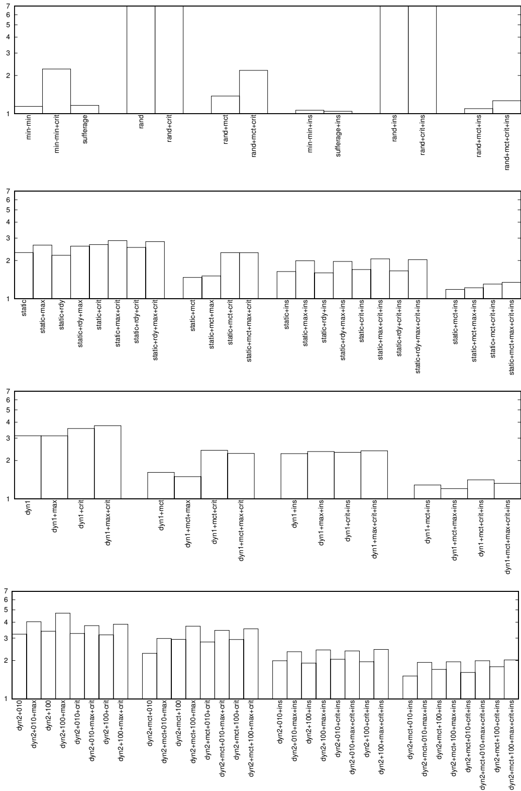
Figure 16: Relative performances of the schedules produced by the different heuristics for platform graphs of type Clique . Average on four types of task graphs, and three communication to computation ratios.
