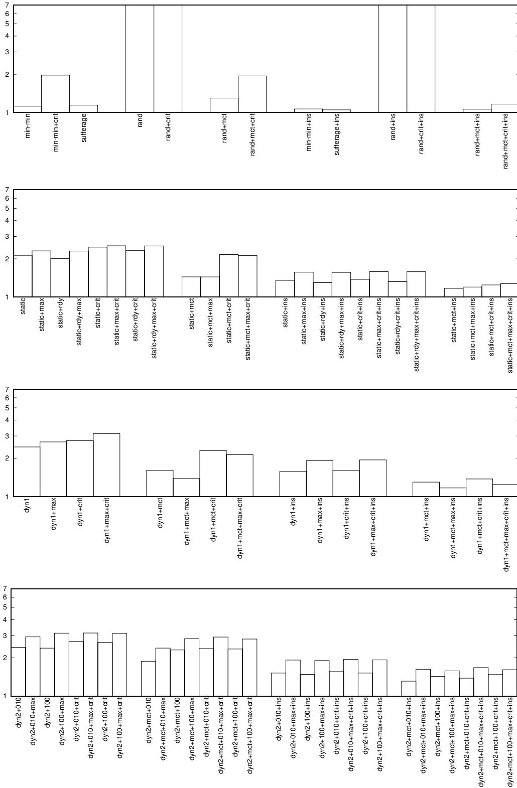
Figure 15: Relative performances of the schedules produced by the different heuristics for communication to computation ratio of 10. Average on four types of task graphs, and three types of platform graphs.
