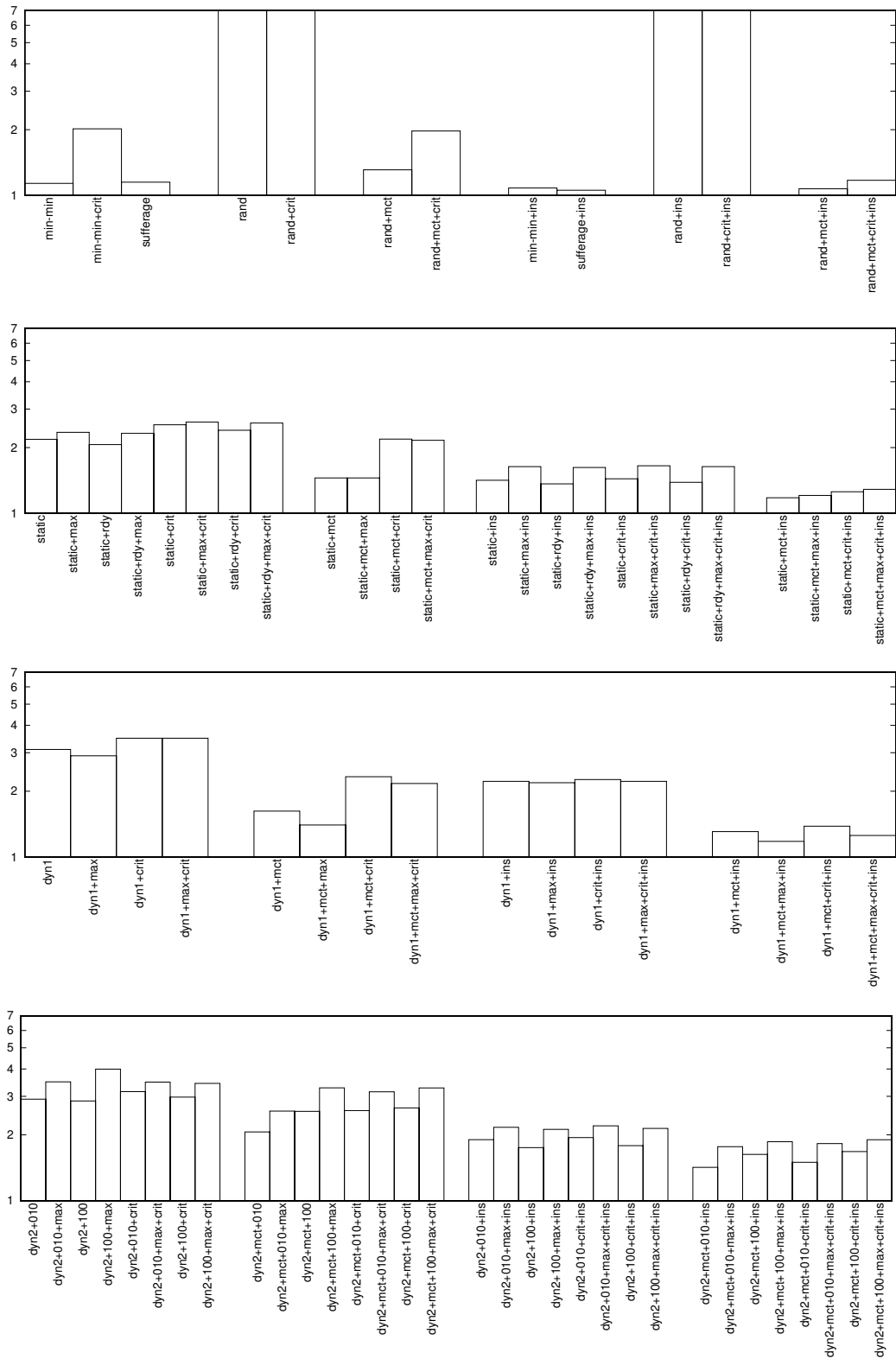
Figure 14: Relative performances of the schedules produced by the different heuristics for communication to computation ratio of 1. Average on four types of task graphs, and three types of platform graphs.
