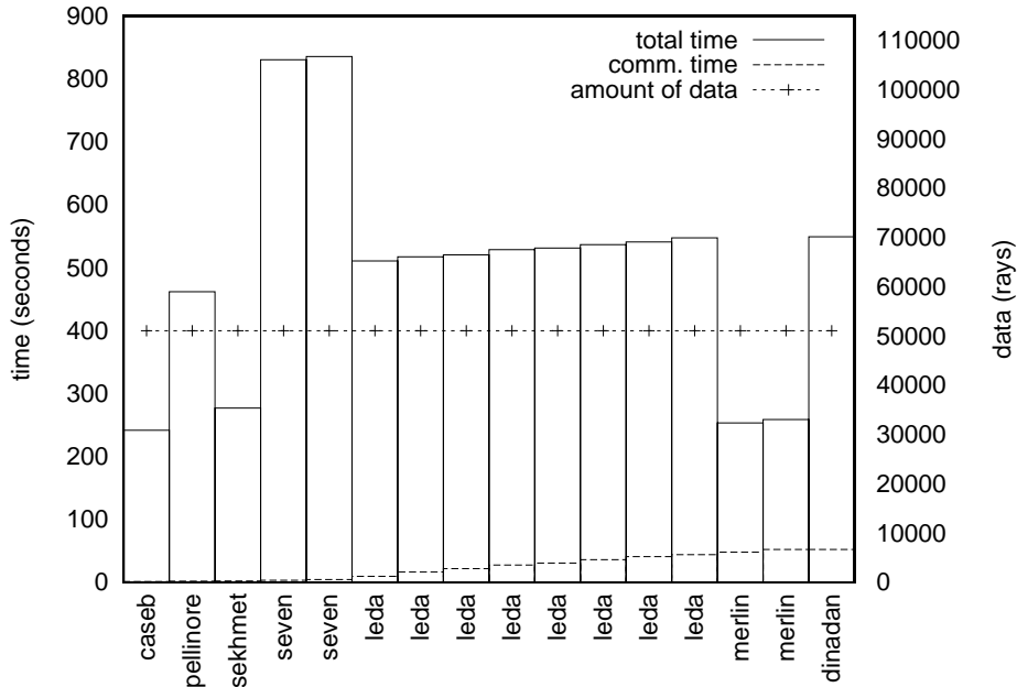
Figure 2: Original program execution (uniform data distribution).
